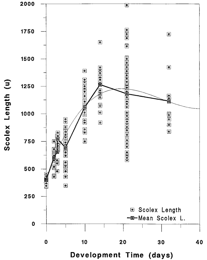
FIGURE 4. Graph of scolex length ( \mu\text{m} ) versus time of development. Growth of strobilae described by the polynomial equation y = 410.63591 + 99.31129x - 3.7688x^2 + 0.04208x^3 ; r^2 = 0.95185 (thin line).
