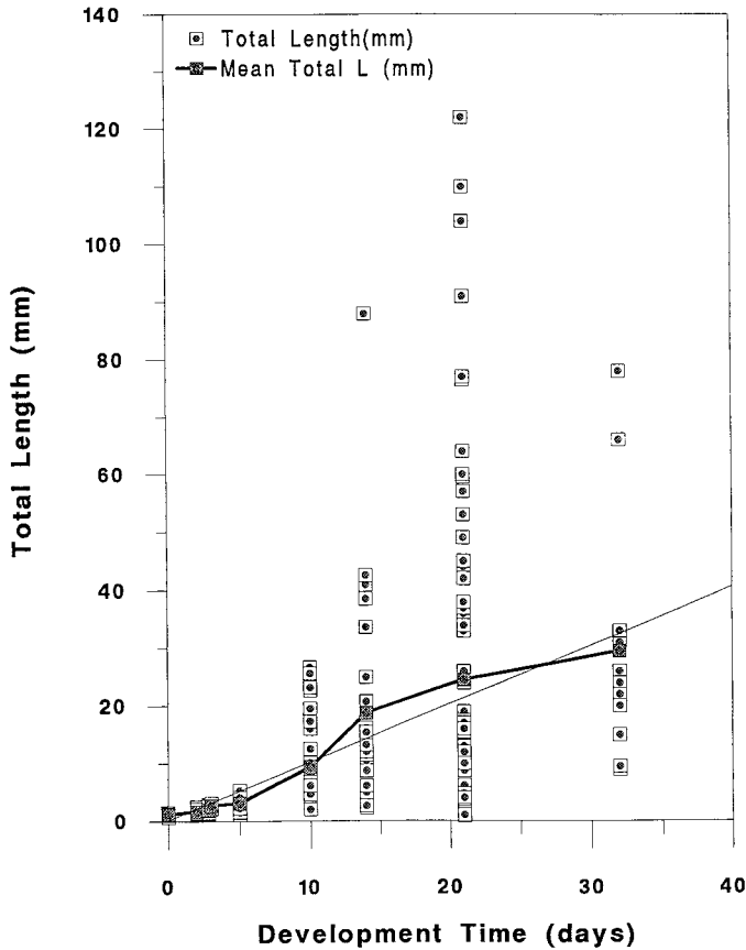
FIGURE 3. Graph of total lengths of strobilae versus time of development. Growth of strobilae described by the linear equation y = 0.23813 + 1.0130x ; r^2 = 0.95254 (thin line).
