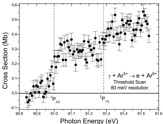
FIG. 1. Photoionization cross-section measurement in the threshold energy region at a spectral resolution of 80 meV. The dashed lines indicate the thresholds of the {}^2P_{1/2} ground state and the {}^2P_{3/2} metastable state determined from these measurements.
