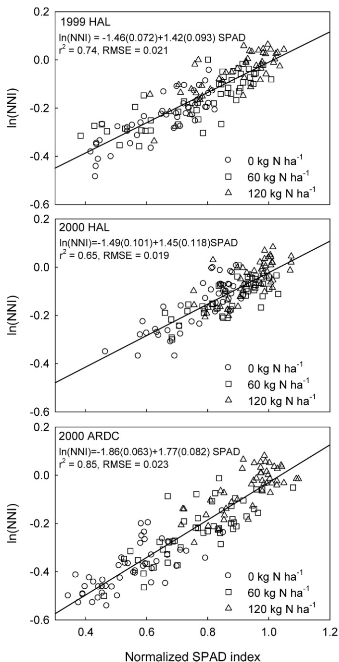
Figure 4. Natural logarithm of the nitrogen nutrition index (NNI) in relation to the normalized SPAD index. \text{NNI} = \%N_a / \%N_c , where \%N_a and \%N_c are the actual and critical N concentration of corn at the R1 stage of development. Critical N concentration was calculated using \%N_c = 3.4 W^{-0.37} , where W was the measured corn shoot biomass (Mg/ha) within that experimental unit. The normalized SPAD index was calculated by dividing the average SPAD reading for each experimental unit by the average SPAD reading across all experimental units within the weed-free, 120-kg N/ha N application treatment within a location.
