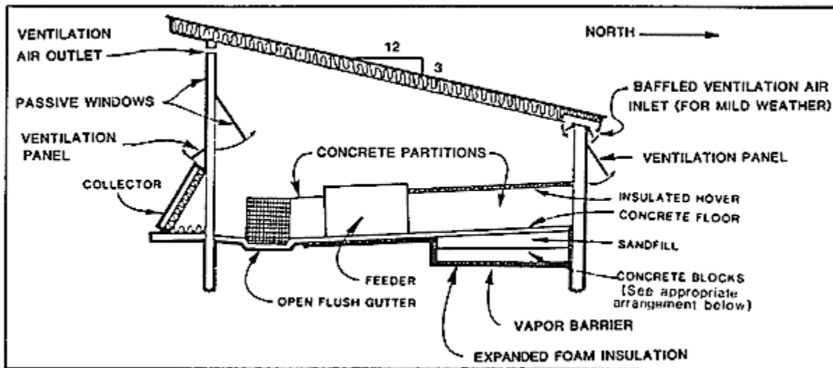
Figure 1. Cross section of the Solar MOF Nursery. Details omitted for clarity.
