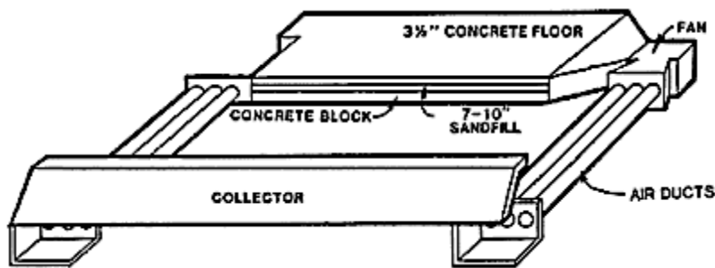
Figure 2. Schematic of the solar collector-in-floor heat distribution-storage system.
