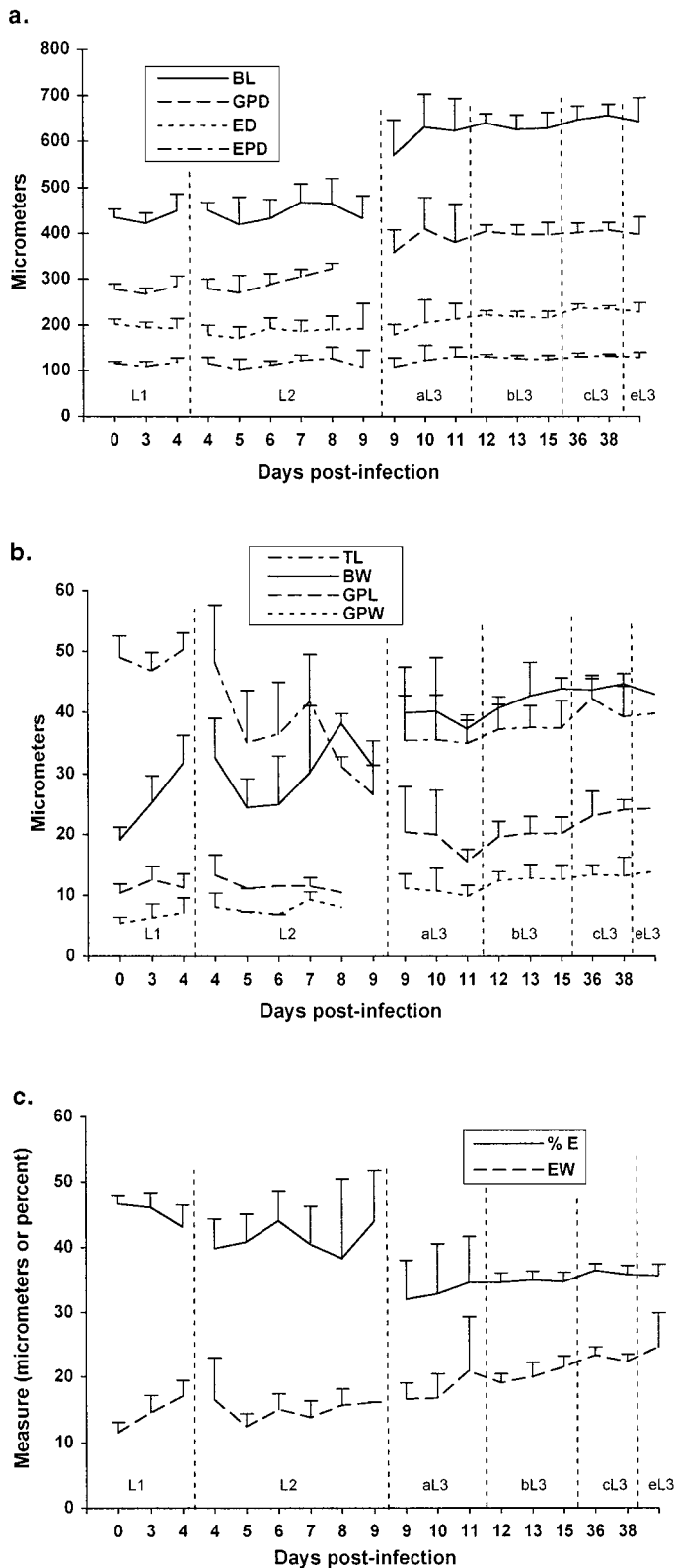
FIGURE 7. (a-c) Mean measurements of larvae of Umingmakstronylus pallikuukensis from Deroceras laeve at 23.4 C at various days postinfection (DPI). L1—first-stage larvae, L2—second-stage larvae, aL3—early thirdstage larvae (L3), bL3—intermediate L3, cL3—late L3, eL3—emerged L3. The 2 sets of data for 4 DPI represent measurements from L1 and L2, and for 9 DPI represent measurements from L2
