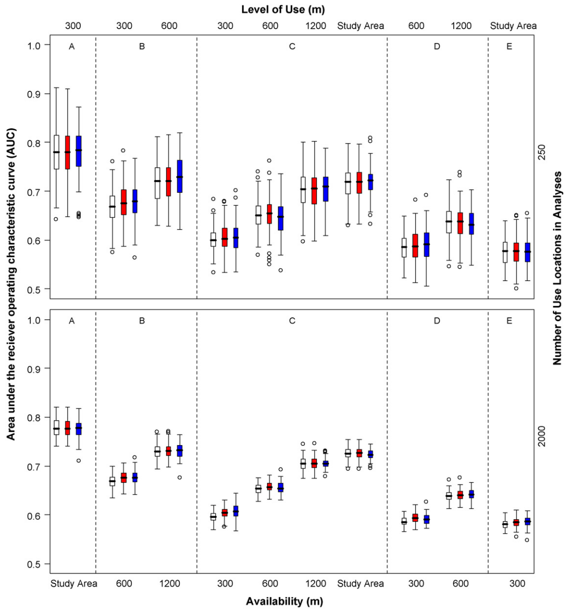
Fig. 3. Area under receiver operating characteristic curve (AUC) scores for discrete-choice (white), logistic-regression (red), and MAXENT models (blue) at sample sizes of 10 or 80 animals with 25 use locations per animal and 5 random locations per use location. Plots are grouped where the ratio between area in which we generated use locations (level of use) and area defined as available was smallest (300 m: study area (A)), 1:2 (B), 1:1 (C), 2:1 (D), and largest (study area: 300 m (E)). Boxes encompass central 50% of observations and length of whiskers = 1.5 × interquartile of the box.
