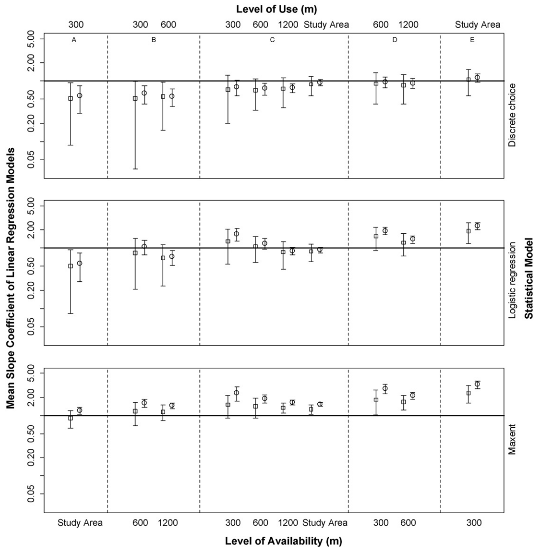
Fig. 2. Mean slope coefficient of linear regression models with known probabilities predicted by estimated probabilities of resource selection and approximate 95% confidence intervals ( \bar{X} \pm 1.96SE ) for discrete-choice, logistic-regression, and Maxent models at sample sizes of 10 ( \square ) or 80 ( \circ ) animals with 25 use locations per animal and 5 random locations per use location. Plots are grouped where the ratio between area in which we generated use locations (level of use) and area defined as available was smallest (300 m: study area (A)), 1:2 (B), 1:1 (C), 2:1 (D), and largest (study area: 300 m (E)).
