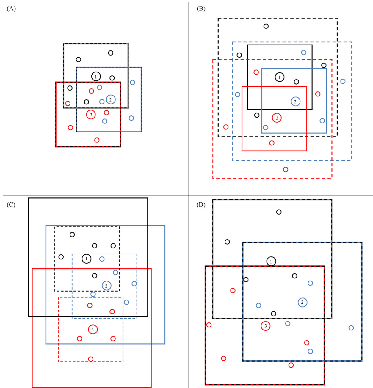
Fig. 1. An illustration of how we generated simulated locations of use (larger black, blue, and red numbered-circles) and random locations (smaller black, blue, and red circles) used in resource selection analyses. In all 4 examples (panels A, B, C, and D), we: (1) generated use locations 1 at a time and chose the first use location (1), according to a known probability distribution, from the set of all possible 30\text{ m} \times 30\text{ m} resource units within the study area; (2) generated use locations 2 and 3 (of the 25/animal simulated in the study) within an area in which we determined use could occur (solid-line boxes), at a minimum distance of 90 m from the previous use location, and sequentially with replacement; and (3) generated 5 random locations/use location within the area we defined to be available (dashed-line boxes). (A) We generated use locations 2 (blue, numbered circle) and 3 (red, numbered circle) within a 600\text{ m} \times 600\text{ m} square area centered on the previous use location (i.e., the animal traveled between 90 m and 300 m prior to recording another use location). We generated random locations within a 600\text{ m} \times 600\text{ m} square area centered on each use location. (B) We generated use locations 2 and 3 within a 600\text{ m} \times 600\text{ m} square area centered on the previous use location and generated random locations within a 1200\text{ m} \times 1200\text{ m} square area centered on each use location. (C) We generated use locations 2 and 3 within a 1200\text{ m} \times 1200\text{ m} square area centered on the previous use location and generated random locations within a 600\text{ m} \times 600\text{ m} square area centered on each use location. (D) We generated use locations 2 and 3 within a 1200\text{ m} \times 1200\text{ m} square area centered on the previous use location and generated random locations within a 1200\text{ m} \times 1200\text{ m} square area centered on each use location. When analyzing the data using discrete choice, the color-coordinated use and random locations were stratified and defined the choice sets. For logistic regression and Maxent, all random locations were evaluated with each use location and defined the choice sets.
