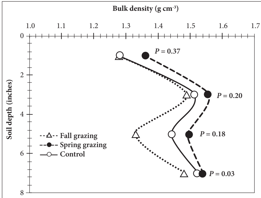
Fig. 2. Soil-depth distribution of bulk density for the 0 to 8 inch depth as affected by 16 years of cattle grazing of corn residues under irrigated no-till system on a Tomak silt loam in eastern Nebraska. The P-values are reported for each depth interval.
