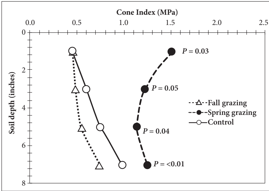
Fig. 1. Soil-depth distribution of cone index (soil compaction parameter) for the 0 to 8 inch depth as affected by 16 years of cattle grazing of corn residues under irrigated no-till system on a Tomak silt loam in eastern Nebraska. The P-values are reported for each depth interval.
