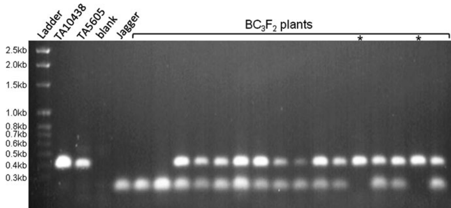
Fig. 1 Co-dominant sequence tagged site (STS) marker pattern of the parents and BC 3 F 2 plants in Jagger background. The STS marker ( Xncw-Lr58-1 ) was based on wheat RFLP marker XksuH16 .
