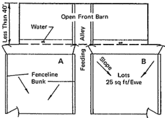
Open-front barn with small lots and fenceline feeding.
