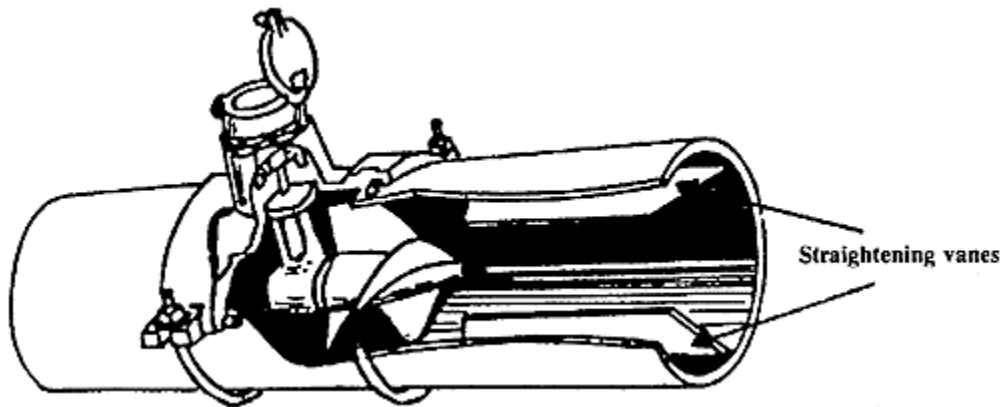
Figure 3. Typical irrigation propeller meter.
