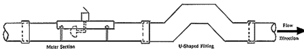
Figure 4. U-shaped fitting installed to guarantee full pipe flow in the meter section.
