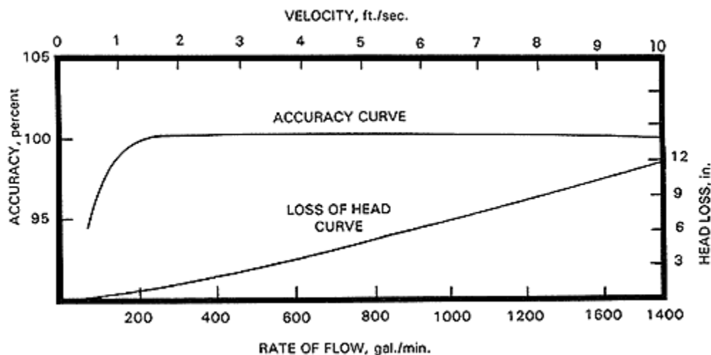
Figure 1. Typical accuracy and head-loss curves for propeller meters.
