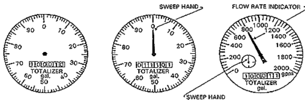
Figure 2. Options available on indicating head.
